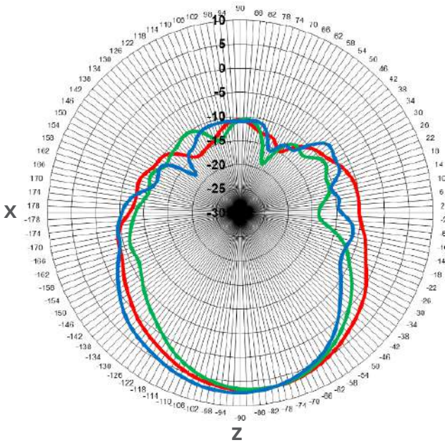
H Plane
